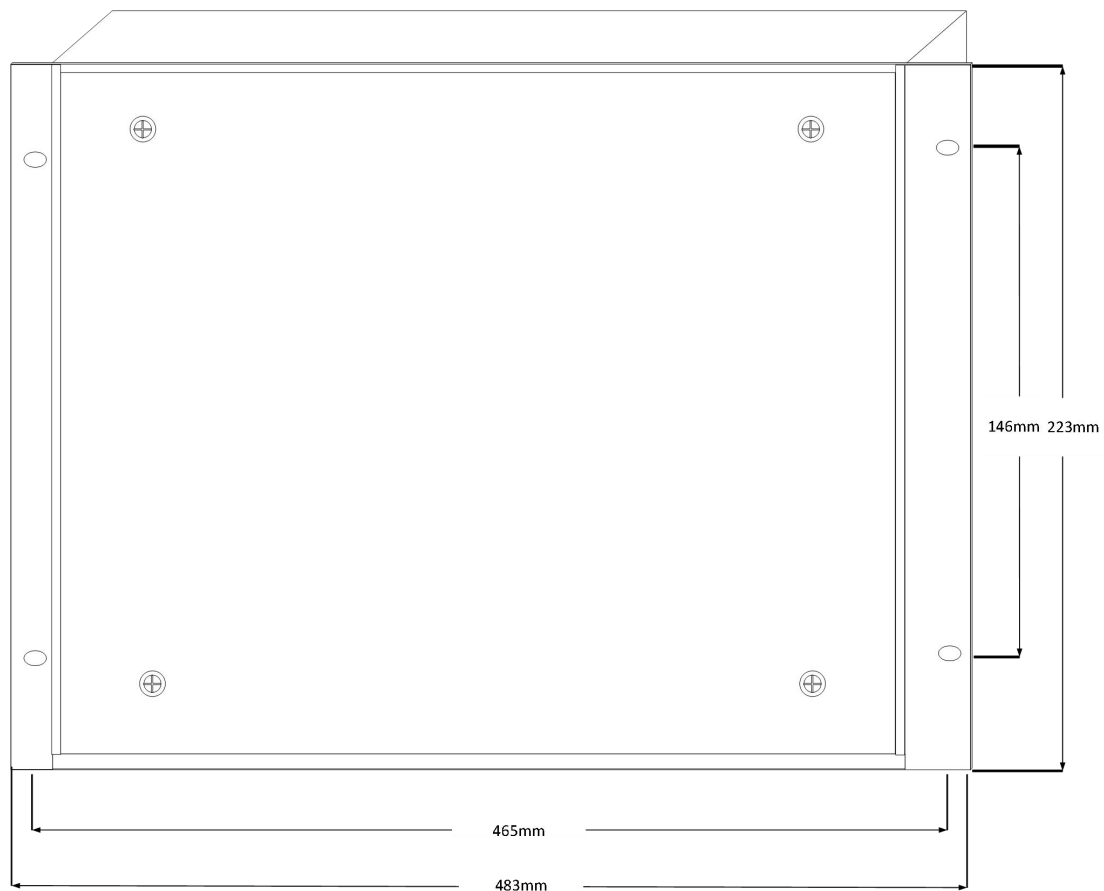
Front panel size diagram
