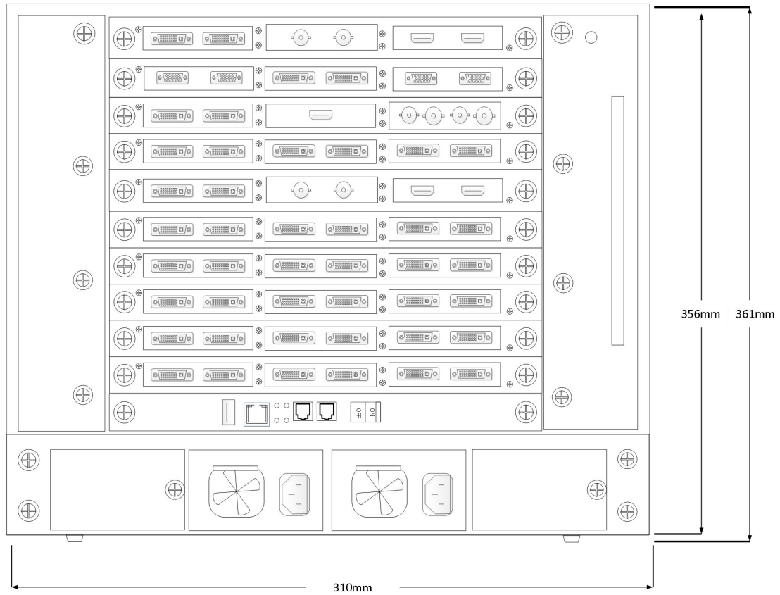
Rear panel size diagram
